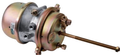
3030 COMPLETE LONGSTROKE CHAMBER W/CLEVIS
